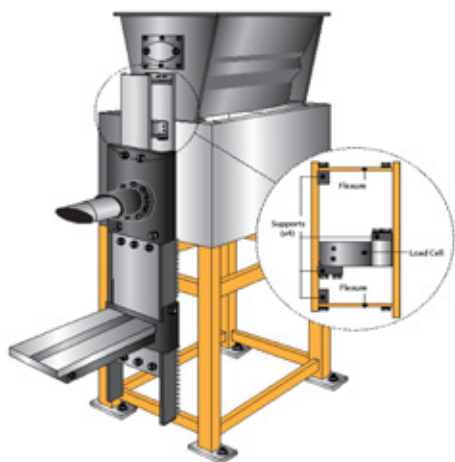
Feed Hopper
