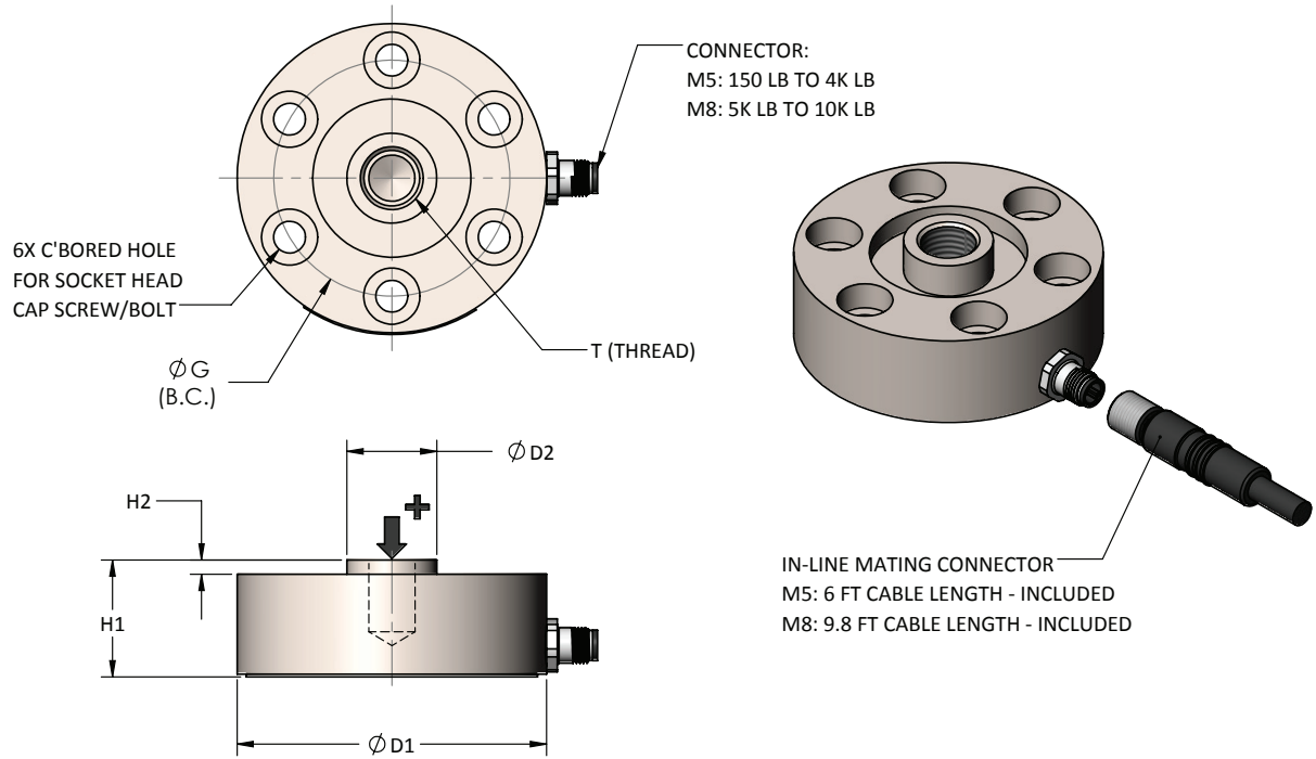
DIMENSIONS IN INCHES
